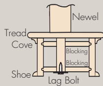
Starting Step Cross Section
